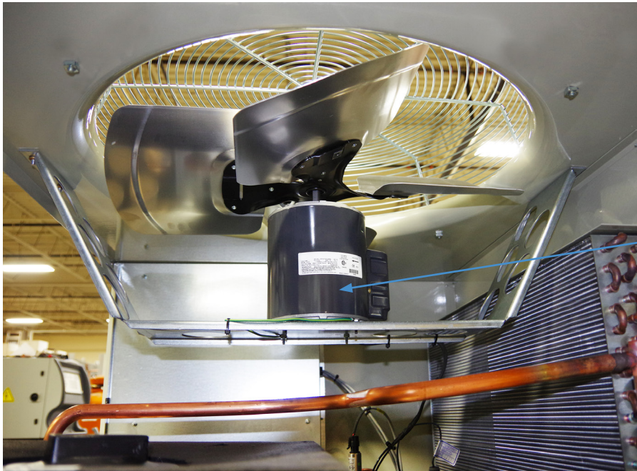
Direct Drive Condenser Fan Motor
